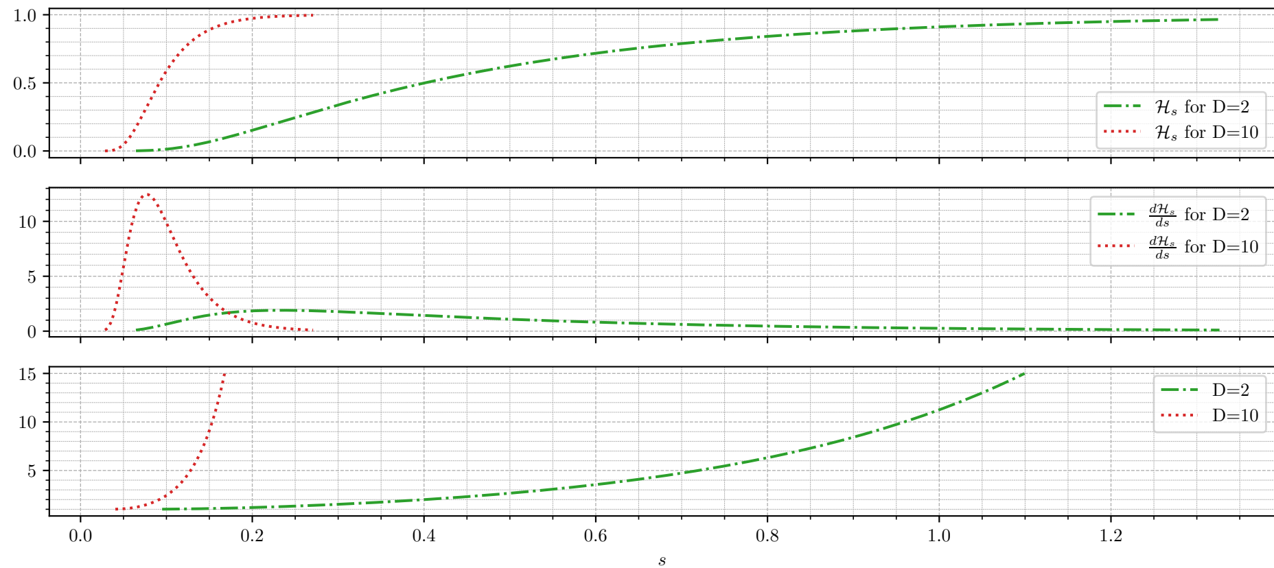
\mathcal{H}_s , its derivative, and number of steps for small dimensions
