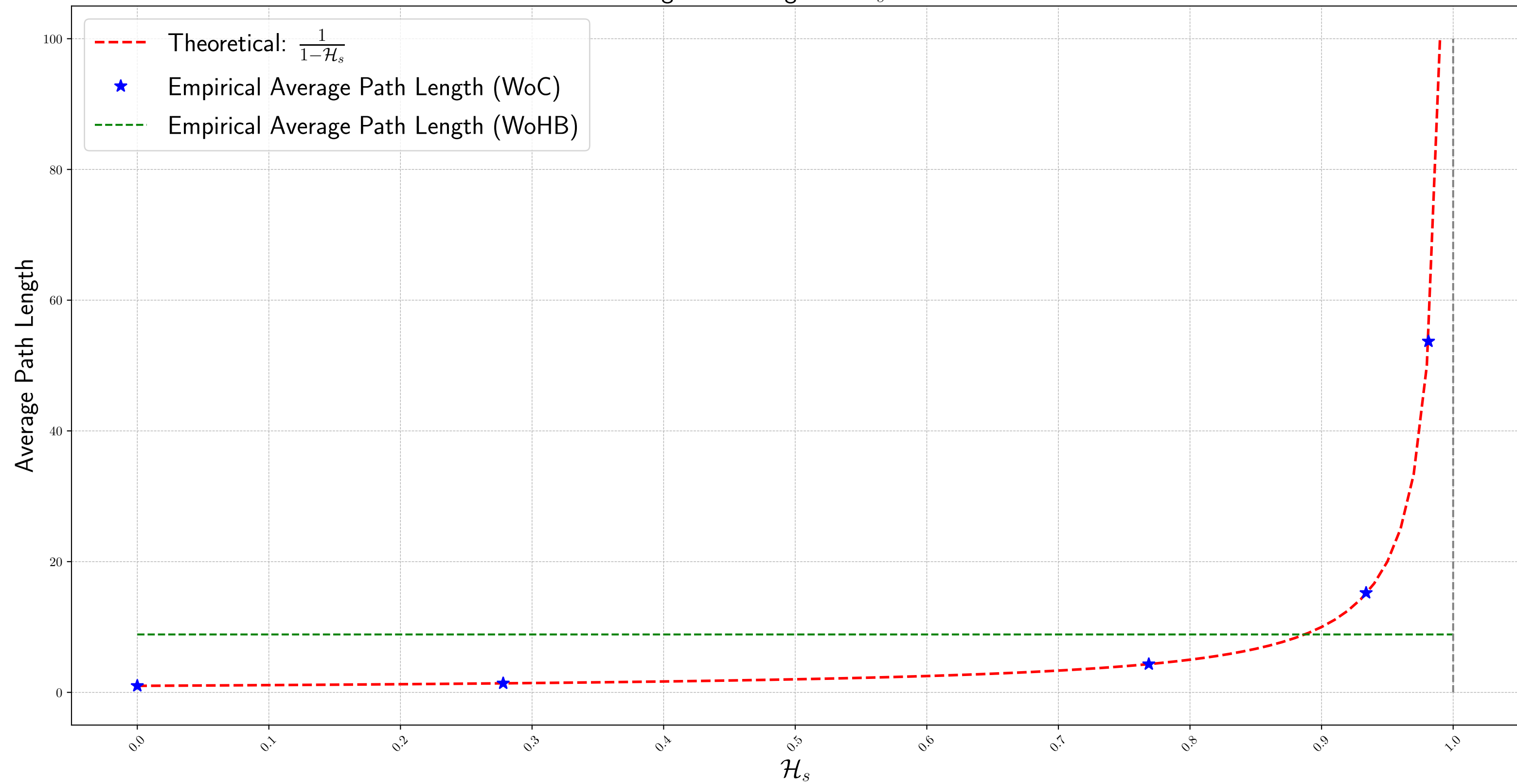
Average Path Length vs \mathcal{H}_s for d = 5
