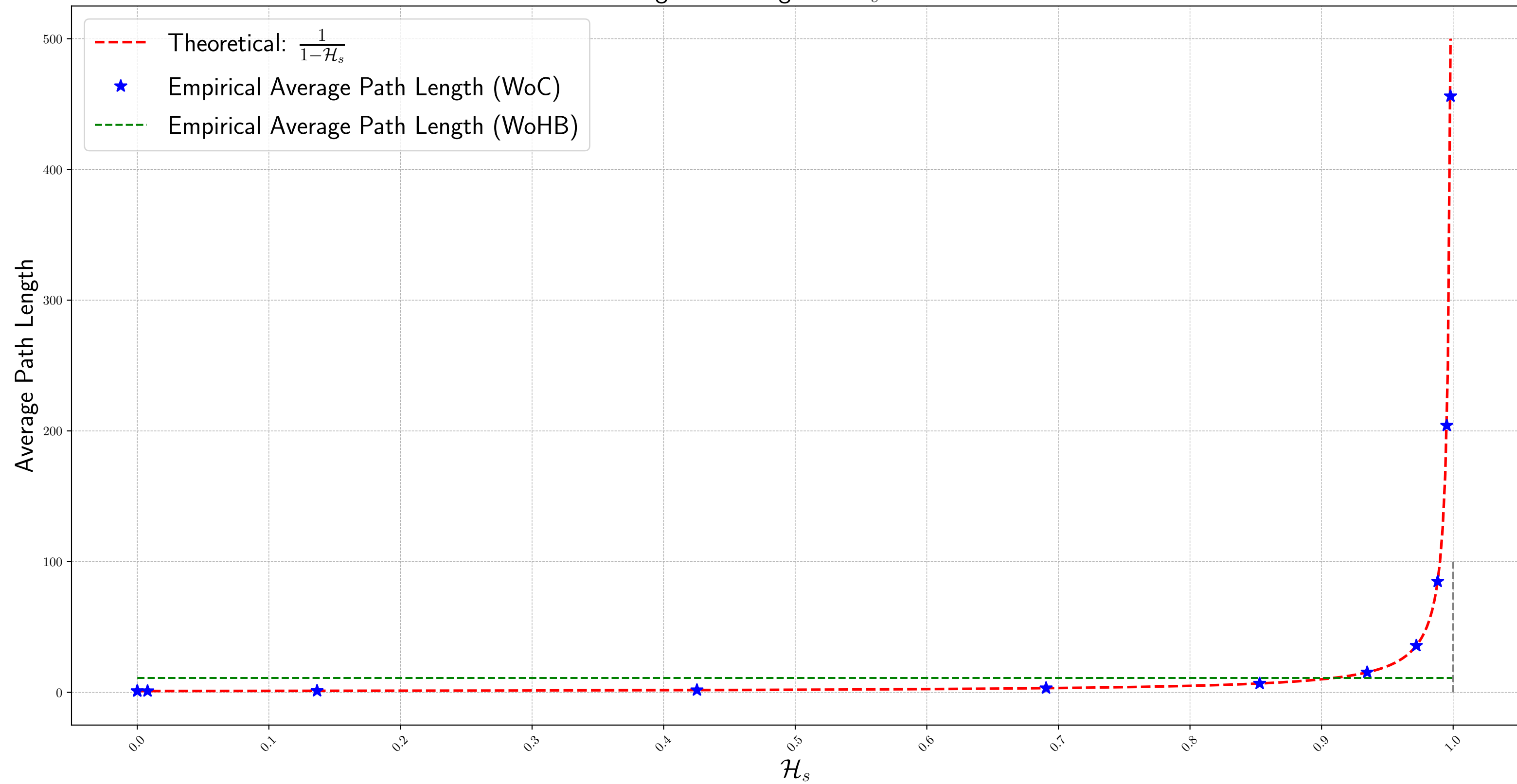
Average Path Length vs \mathcal{H}_s for d = 20
