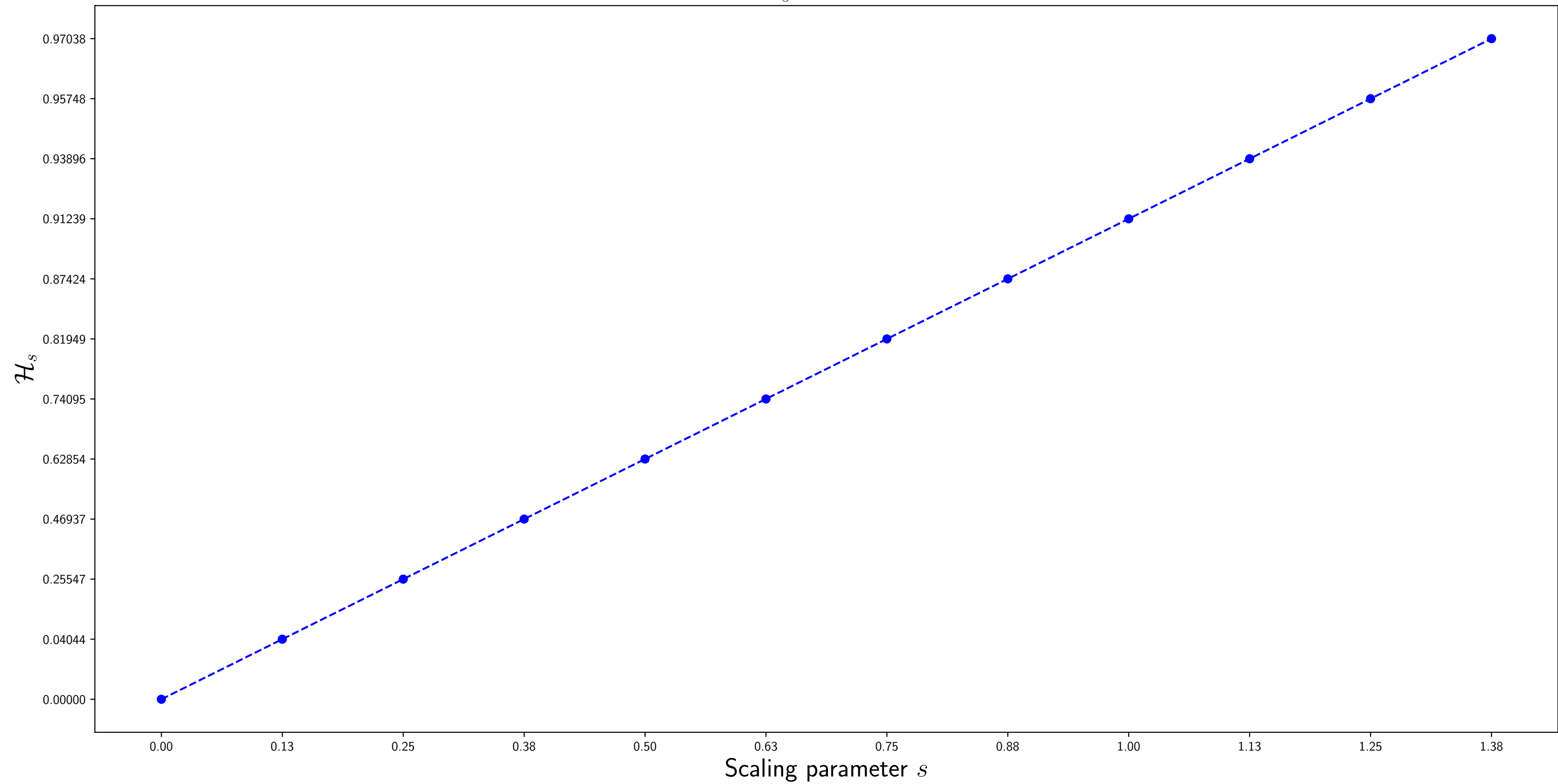
\mathcal{H}_s for d = 2
