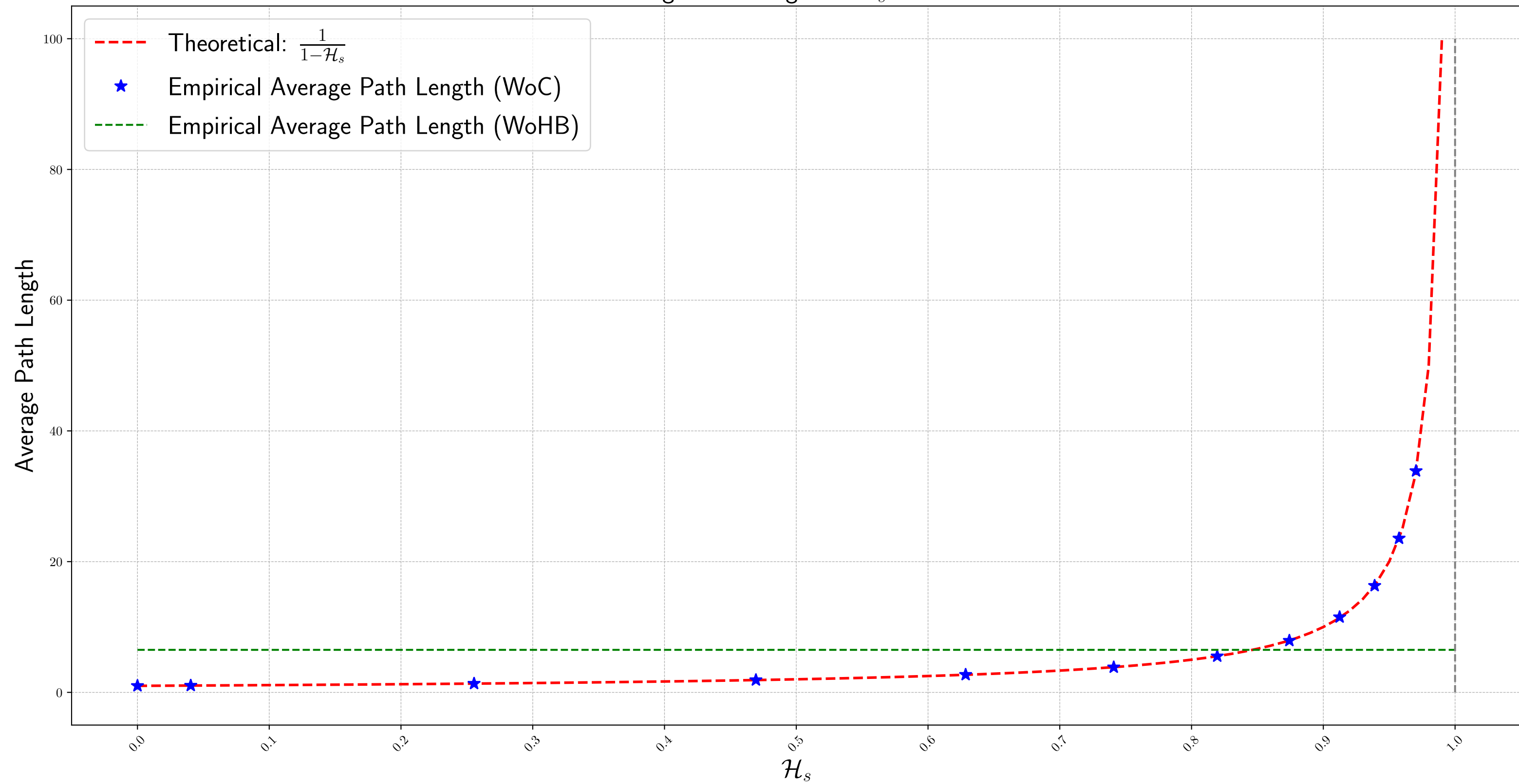
Average Path Length vs \mathcal{H}_s for d = 2
