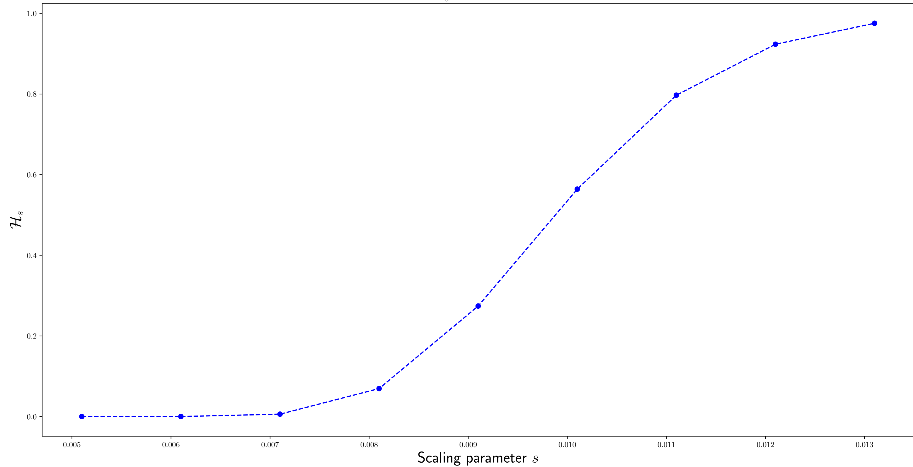
\mathcal{H}_s for d = 100
