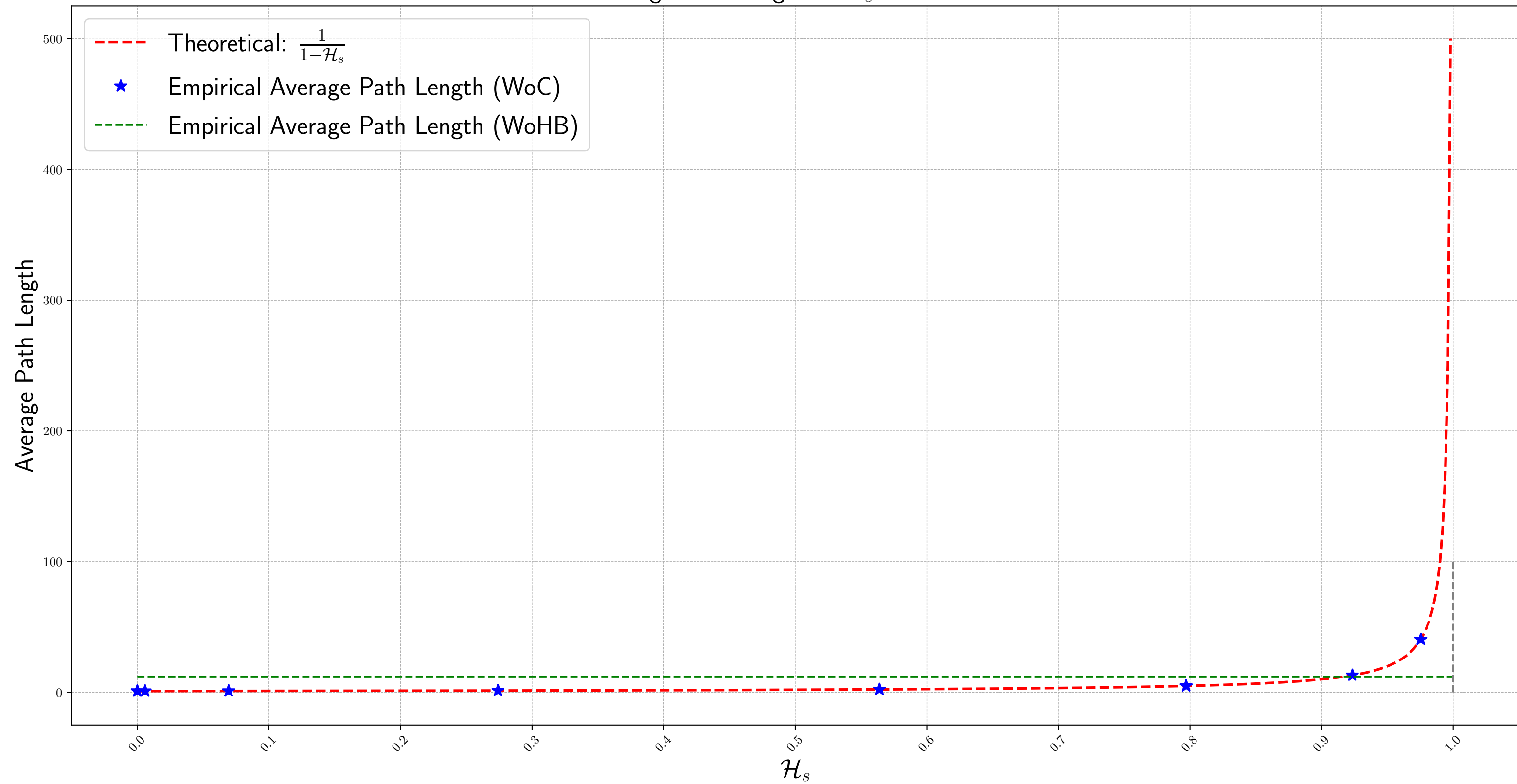
Average Path Length vs \mathcal{H}_s for d = 100
