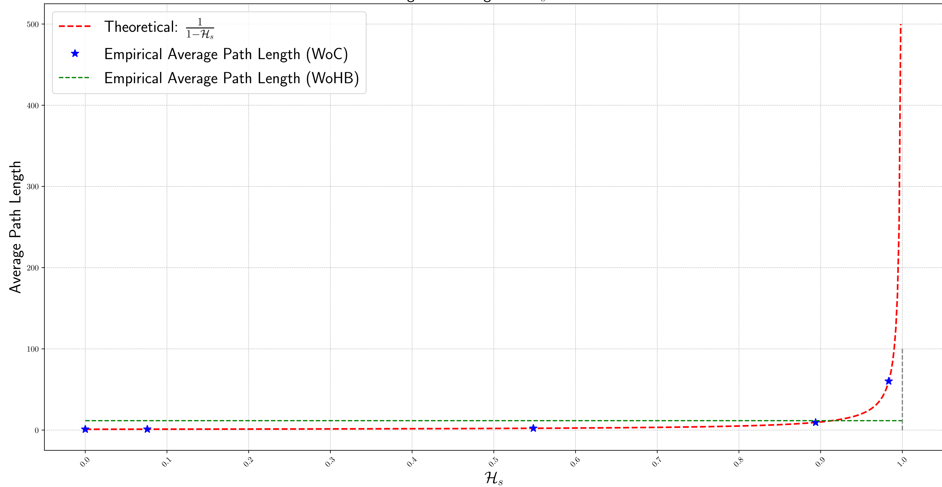
Average Path Length vs \mathcal{H}_s for d = 50
