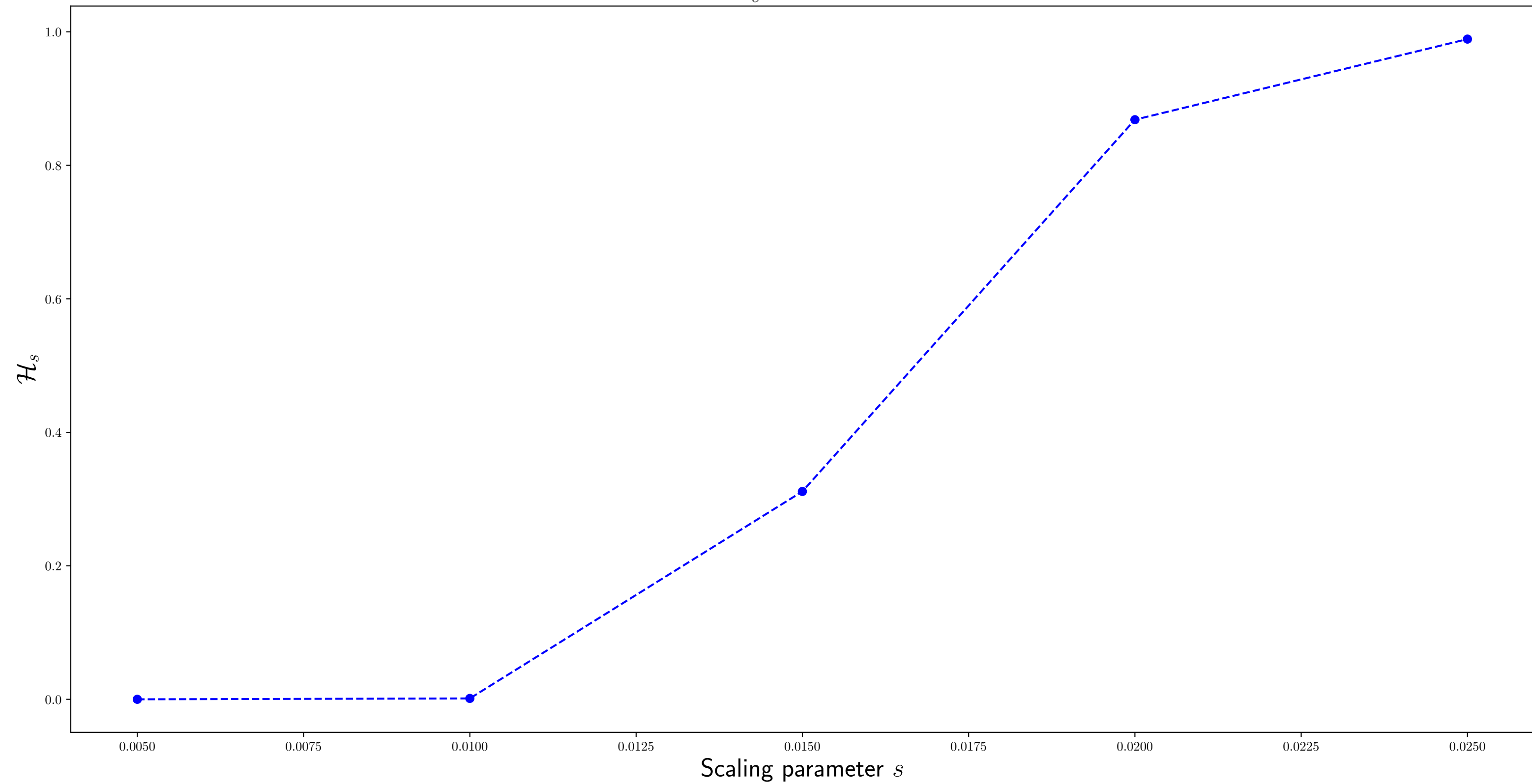
\mathcal{H}_s for d = 60
