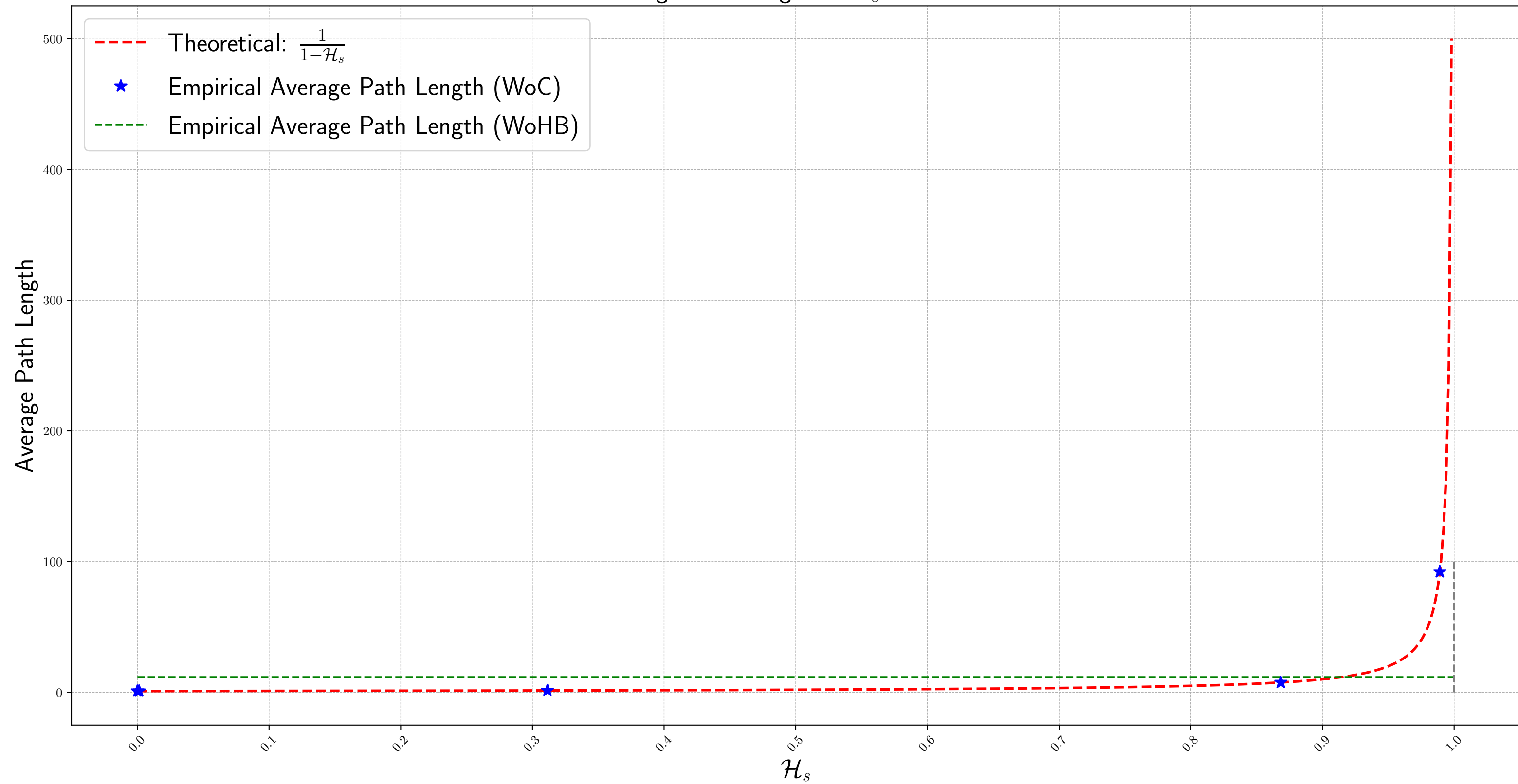
Average Path Length vs \mathcal{H}_s for d = 60
