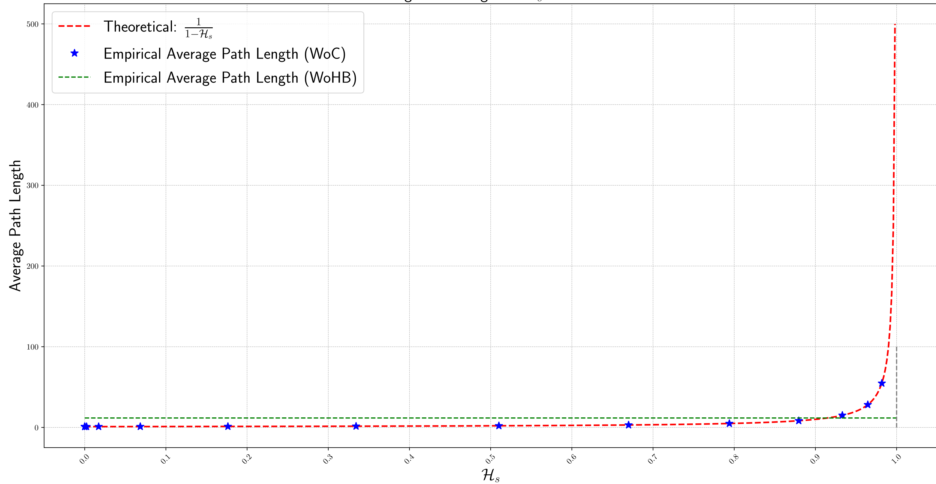
Average Path Length vs \mathcal{H}_s for d = 70
