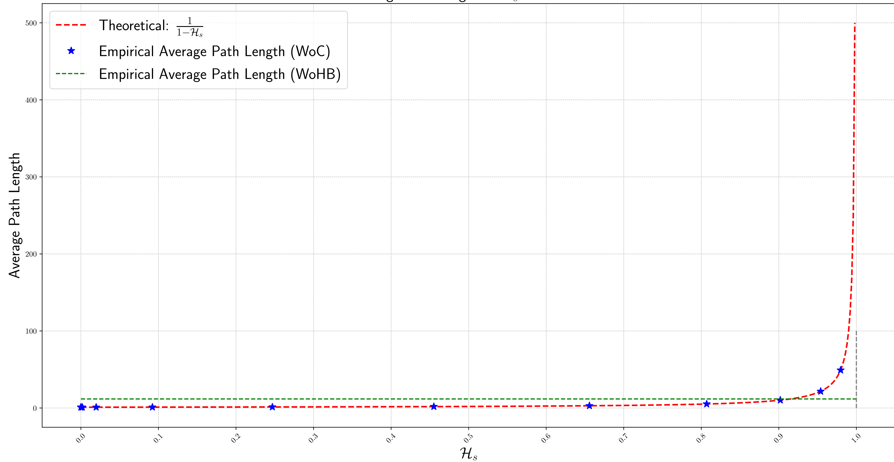
Average Path Length vs \mathcal{H}_s for d = 80
