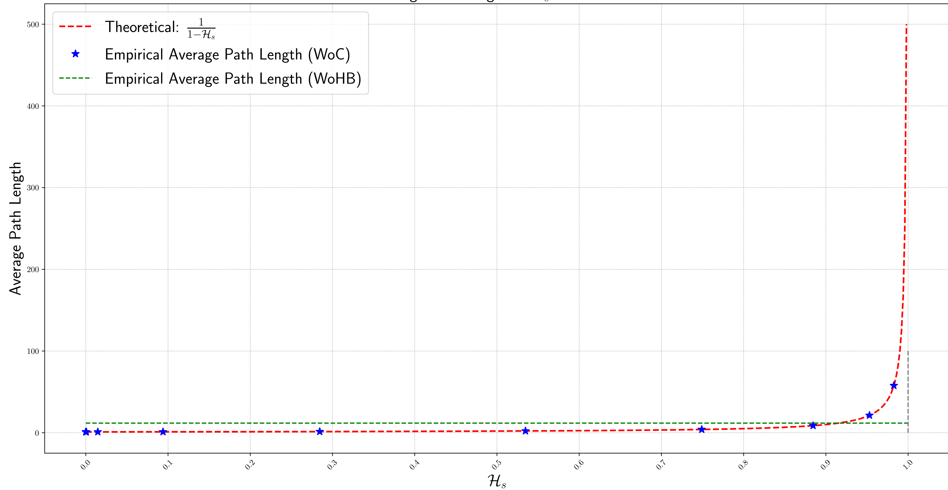
Average Path Length vs \mathcal{H}_s for d = 90
