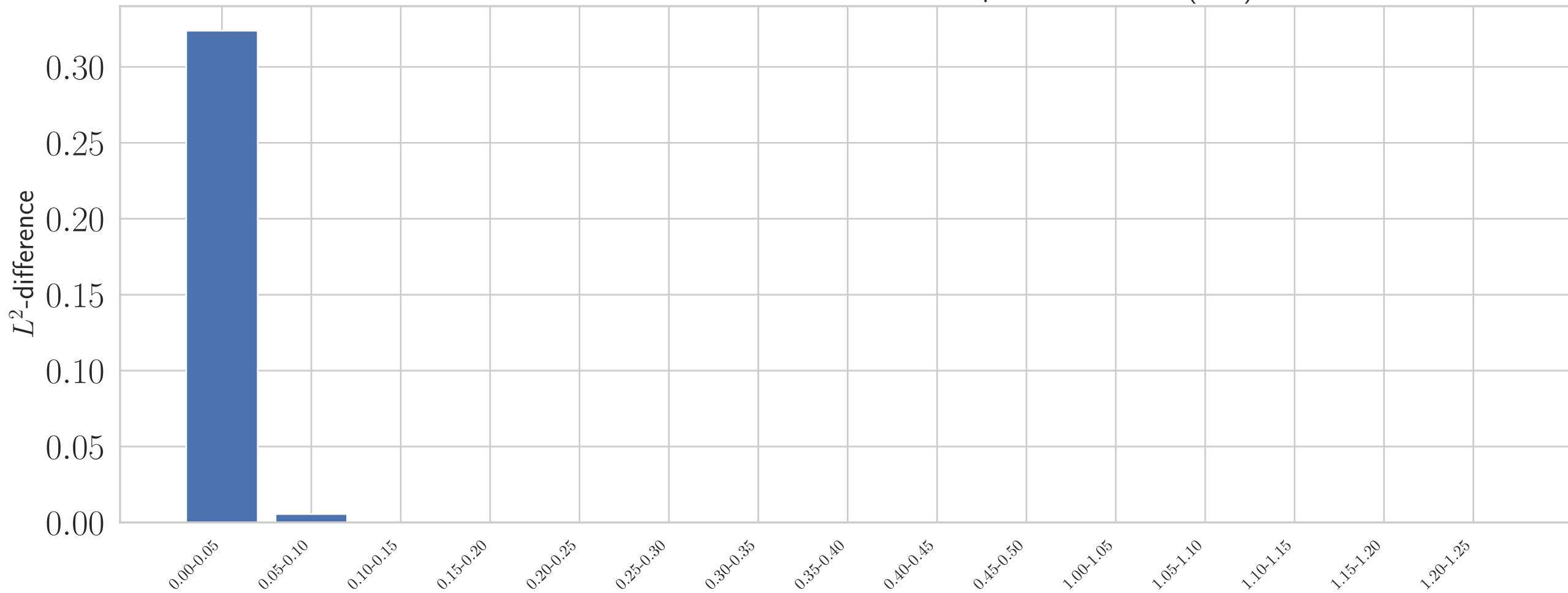
L^2 difference between consecutive fine time-step value functions (ms1)
