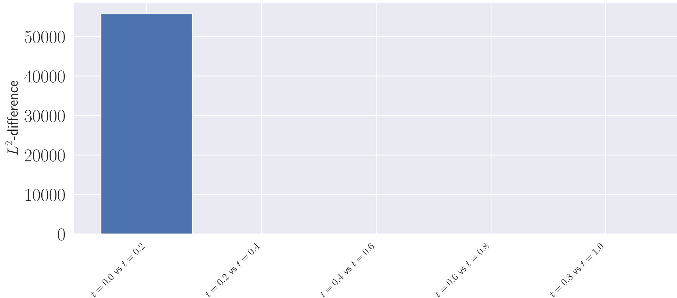
L^2 difference between consecutive coarse time-step value functions
