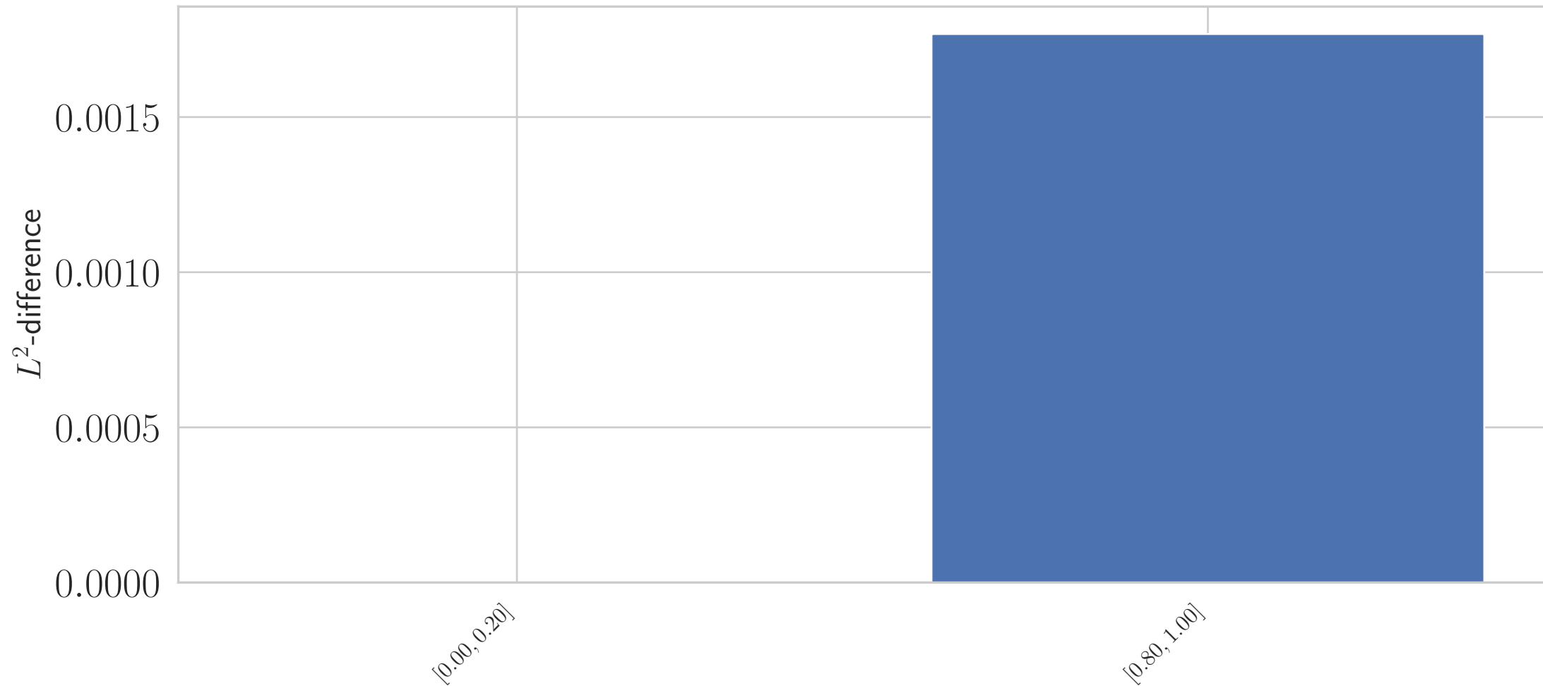
L^2 difference across each ms1 interval
