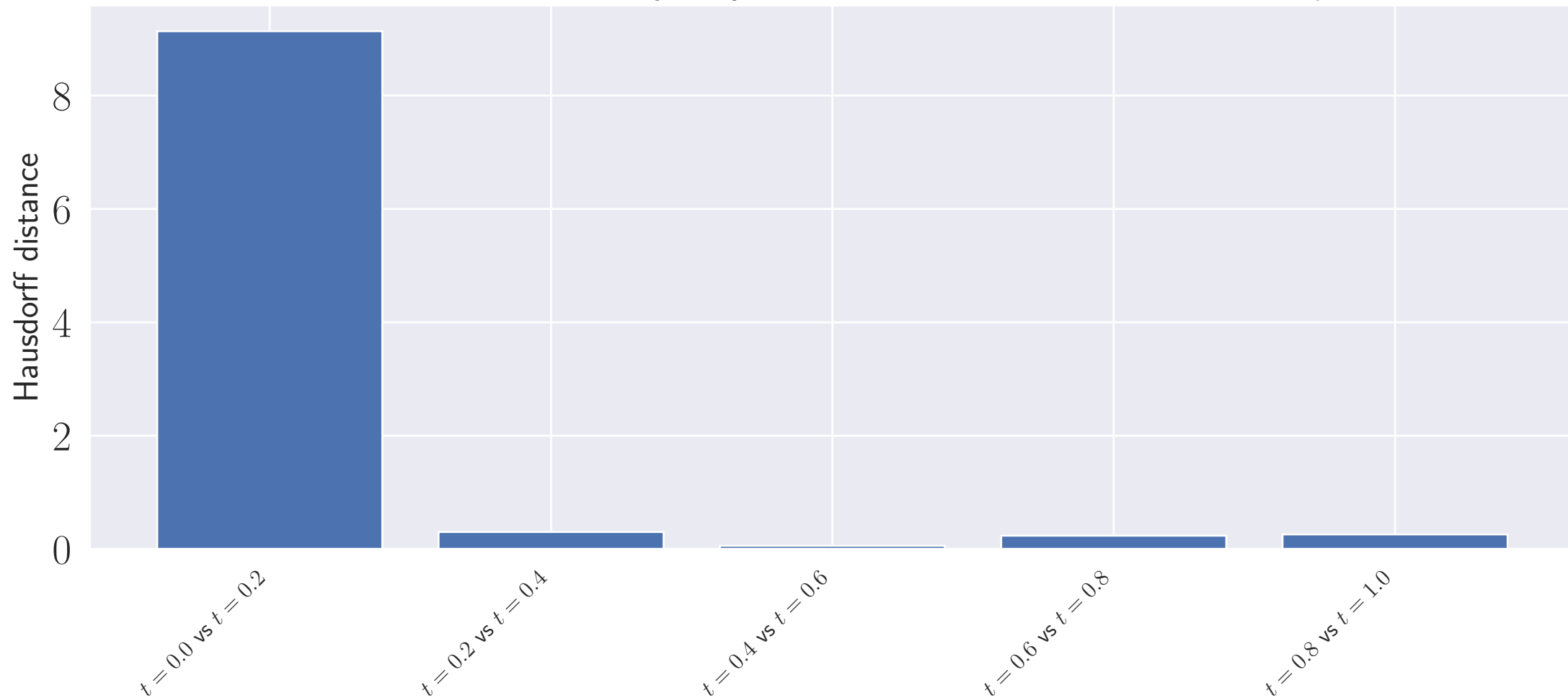
Hausdorff distance of trajectory data between consecutive coarse time steps
