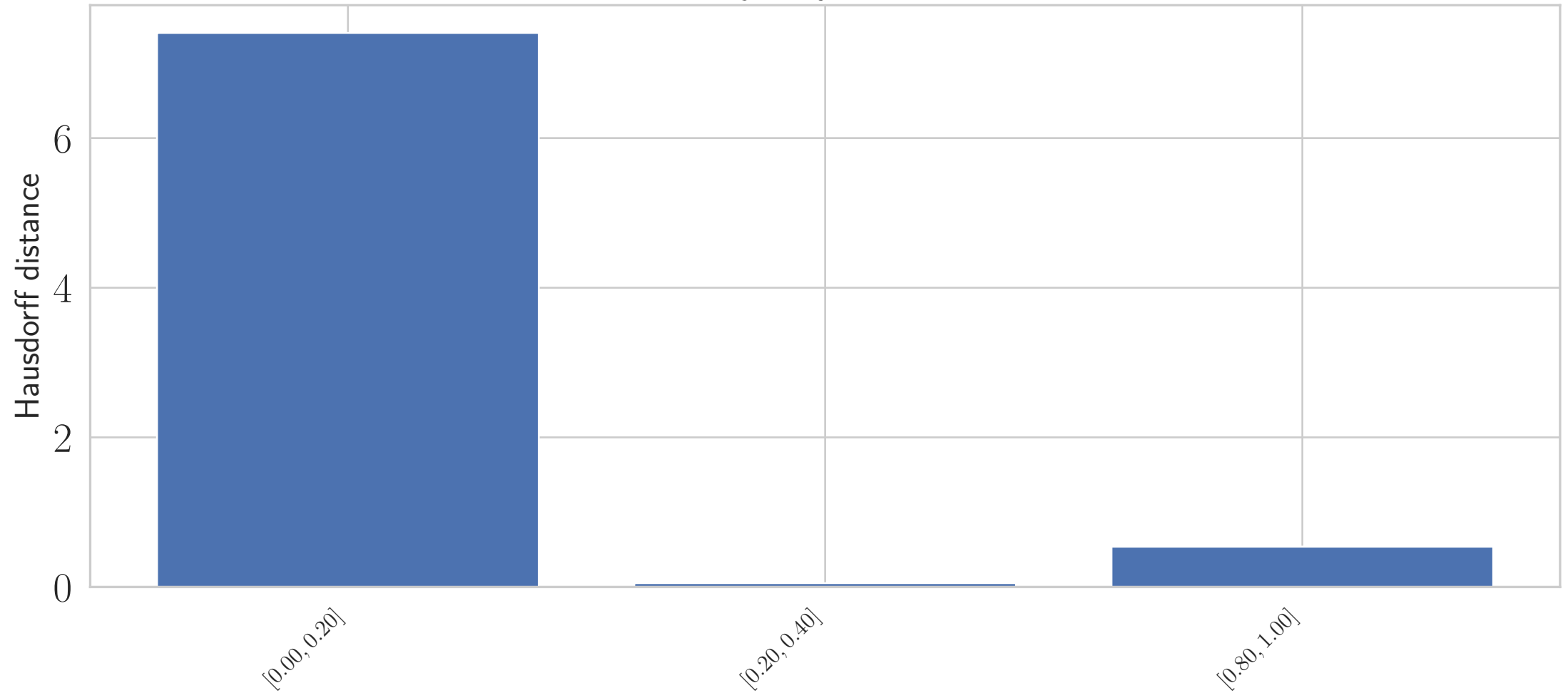
Hausdorff distance of trajectory data across each ms1 interval
