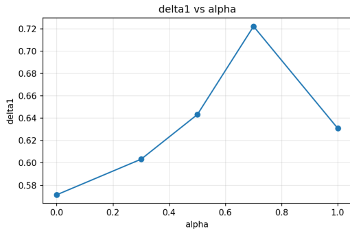
\delta_1 vs \alpha ( \uparrow better)
