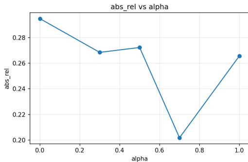
AbsRel vs \alpha ( \downarrow better)
