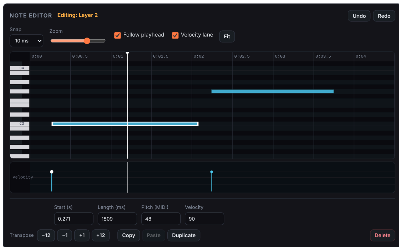
The note editor with one note selected.
