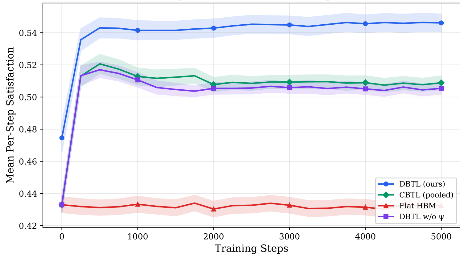
Expanded 8-Recipe LOO: Aggregate Learning Curves (8 held-out splits \times 10 seeds = 80 runs per method)
