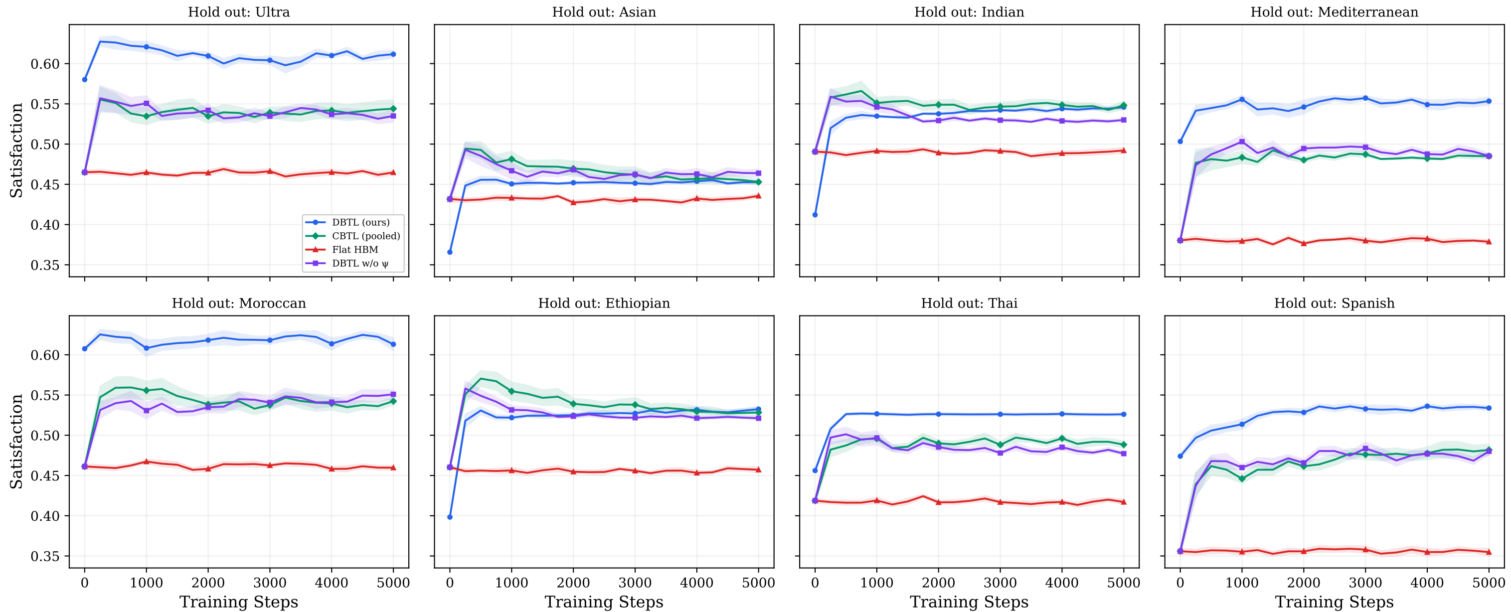
Expanded 8-Recipe LOO: Per-Split Learning Curves (10 seeds)
