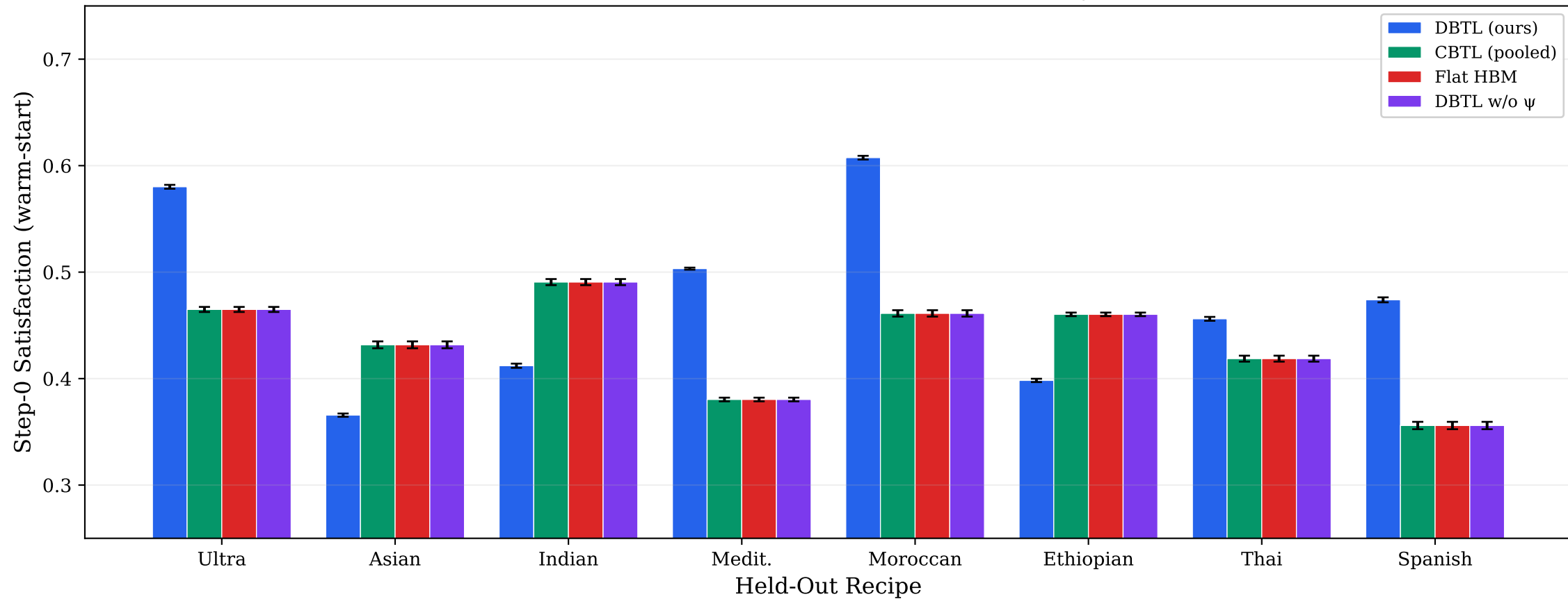
Expanded 8-Recipe LOO: Warm-Start Transfer Quality (10 seeds)
