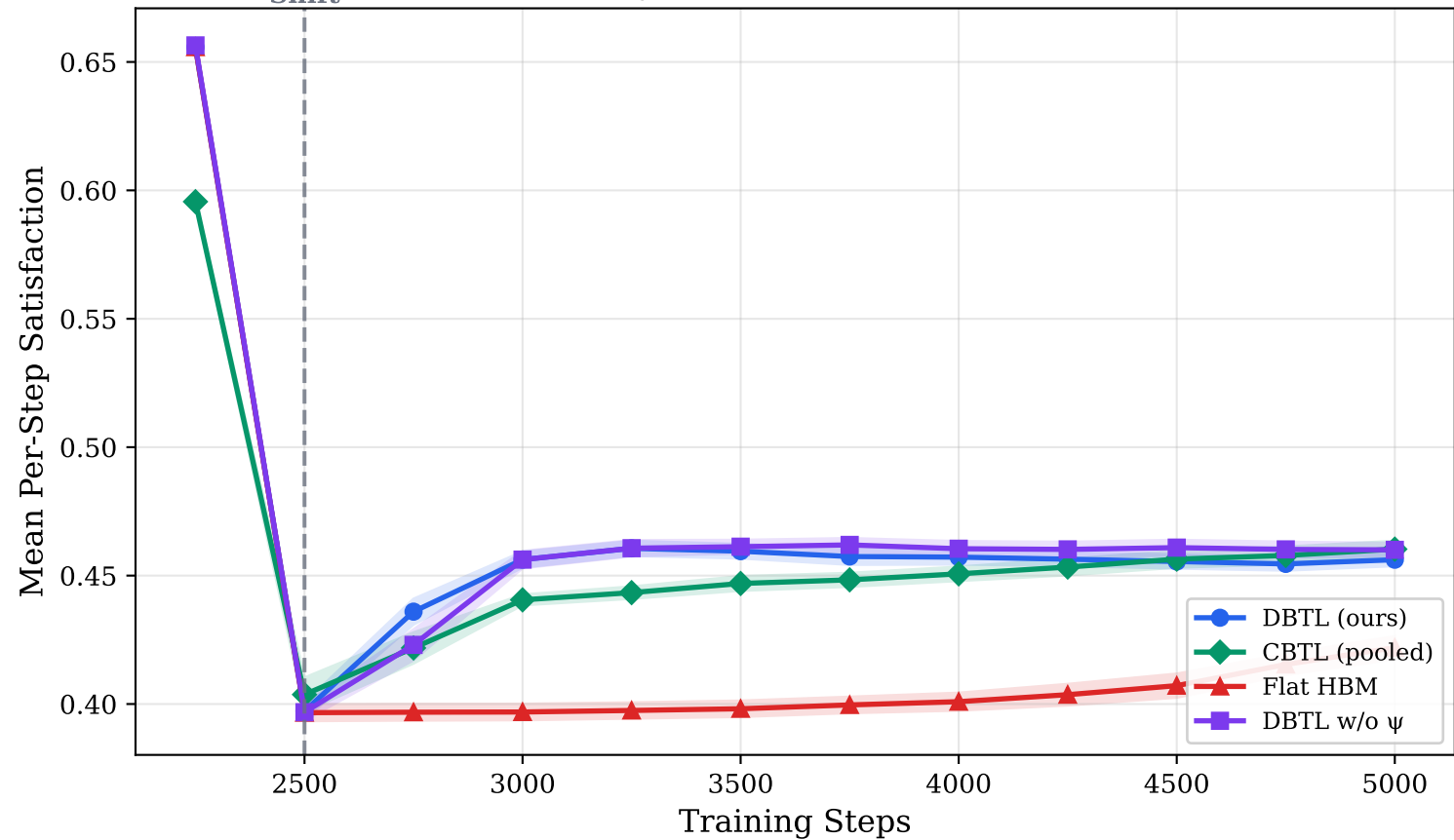
Post-Shift Recovery Detail (steps 2250–5000, 10 seeds)
