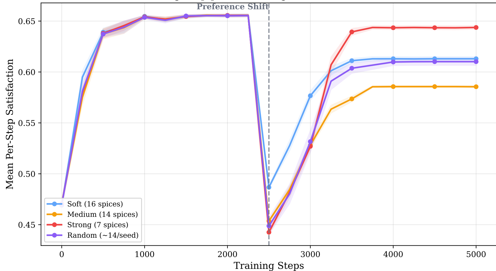
DBTL Recovery: Soft vs Medium vs Strong vs Random Shifts (sign-flip preserves magnitude, 10 seeds)
