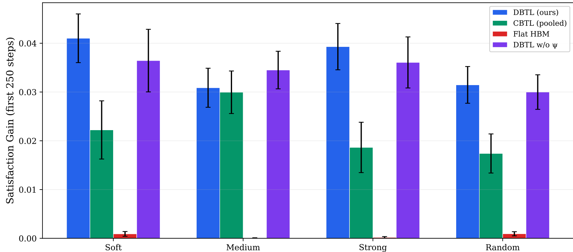
Early Recovery Speed: Satisfaction Gain in First 250 Steps Post-Shift (10 seeds)
