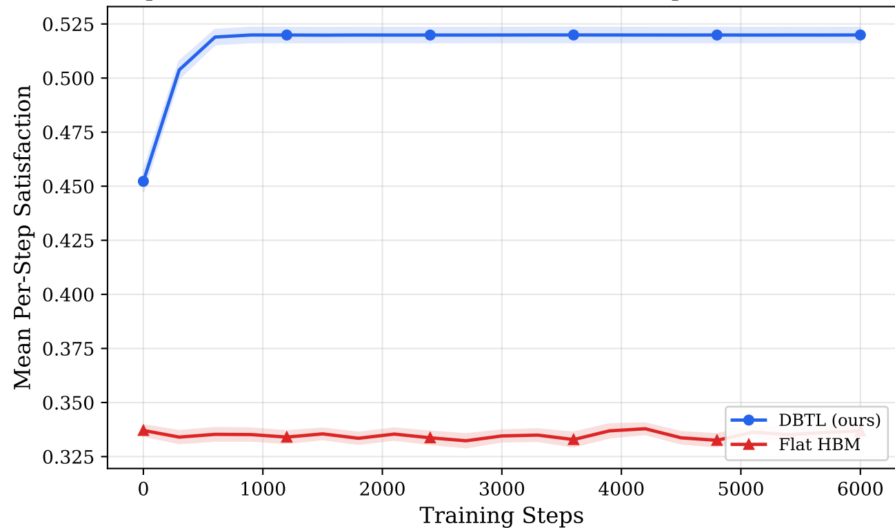
SpiceEnv: Middle-Eastern LOO Transfer (4 splits \times 10 seeds)
