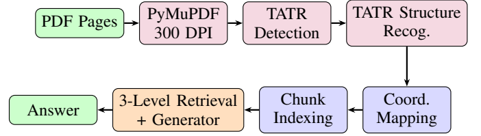
Fig. 2. TableTransformerRAG pipeline: DETR-based visual table detection and structure recognition (TATR), pixel-to-PDF-point coordinate mapping, and the shared three-level retrieval and symbolic-neural generation stack.
