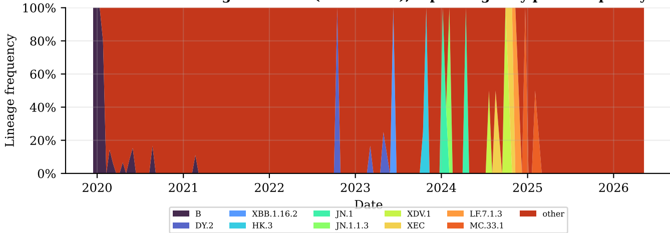
SARS-CoV-2 lineage turnover (Nextstrain), top lineages by peak frequency
