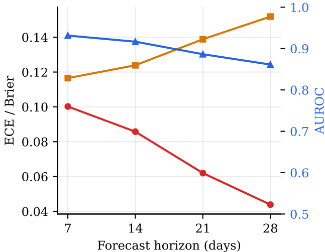
Calibration vs. horizon
