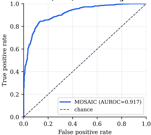
ROC: P(R_t > 1) vs. realised growth
