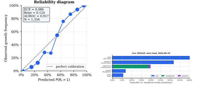
Figure 2: Left: reliability diagram of \mathbb{P}(R_t > 1) over 1,334 forecasts on the NWSS record ( \text{ECE} = 0.086 , Brier 0.124, AUROC 0.917). Right: live alert feed, fused \mathbb{P}(R_t > 1) stacked by stream contribution; SARS-CoV-2 is wastewater-driven, the rest text-driven.
