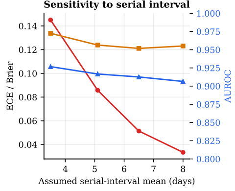
Figure 8: Sensitivity of calibration to the assumed serial-interval mean. Discrimination is invariant; calibration shifts smoothly from over- to under-confidence, with the literature value (5.1 d) well-calibrated.
