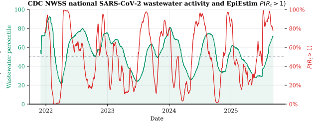
Figure 1: Wastewater nowcasting on real CDC NWSS data. National mean percentile (green) and EpiEstim \mathbb{P}(R_t > 1) (red), 2021–2025. The growth probability leads each wave.
