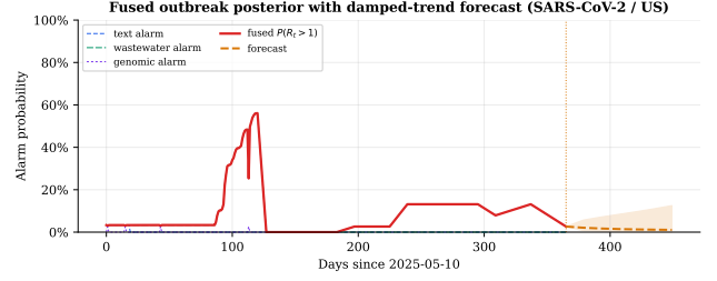
Figure 5: Fused posterior and forecast (SARS-CoV-2 / US). Per-stream alarms (dashed) and the fused \mathbb{P}(R_t > 1) (solid red), with the damped-trend forecast (orange) and its 95% band beyond the last observation.
