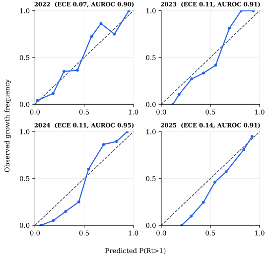
Figure 9: Per-year reliability diagrams ( h=14 ). The curves track the diagonal in every year, confirming the calibration is not an artefact of one era.
