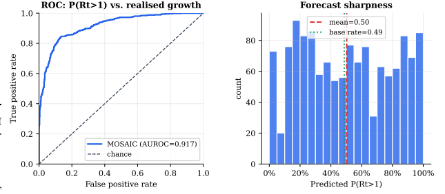
Figure 6: Left: ROC curve of \mathbb{P}(R_t > 1) against realised growth (AUROC 0.917). Right: histogram of predicted probabilities (sharpness); the distribution is bimodal and its mean matches the base rate.
