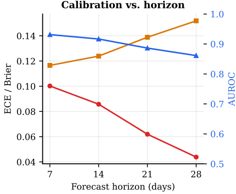
Figure 7: Calibration versus forecast horizon. ECE and Brier (left axis), AUROC (right axis). Longer horizons are easier to calibrate but harder to discriminate.
