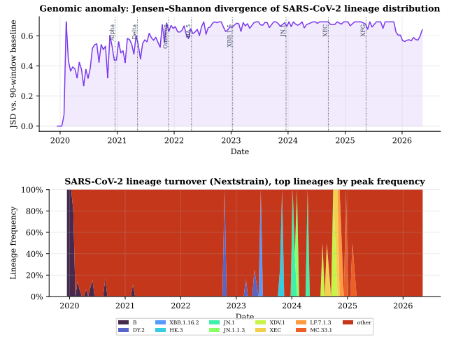
Figure 3: Genomic stream. Top: Jensen–Shannon divergence of the SARS-CoV-2 lineage distribution (real Nextstrain snapshots) with documented variant-emergence dates. Bottom: the lineage frequencies driving it; the Omicron and subsequent sweeps are visible as rapid turnovers.
