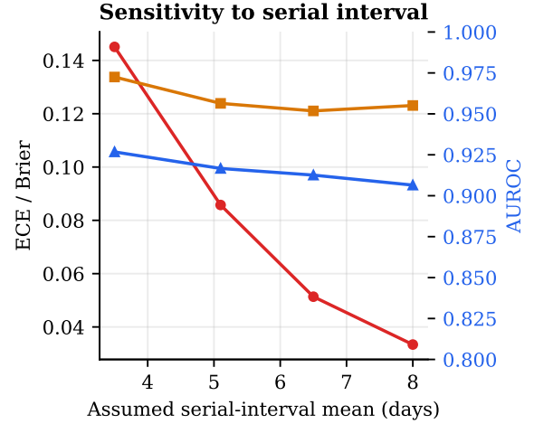
Figure 9: Sensitivity of calibration to the assumed serial-interval mean. Discrimination is invariant; calibration shifts smoothly from over- to under-confidence, with the literature value (5.1 d) well-calibrated.
