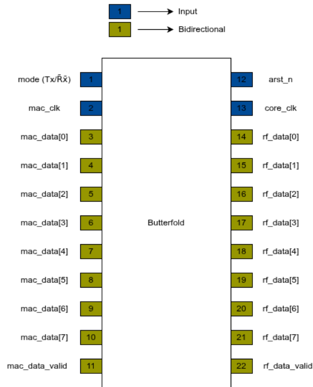
Figure 2: Expected pinout
