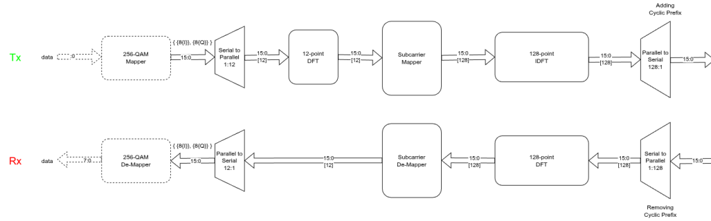
Figure 3: Folded PHY Top Level Architecture
