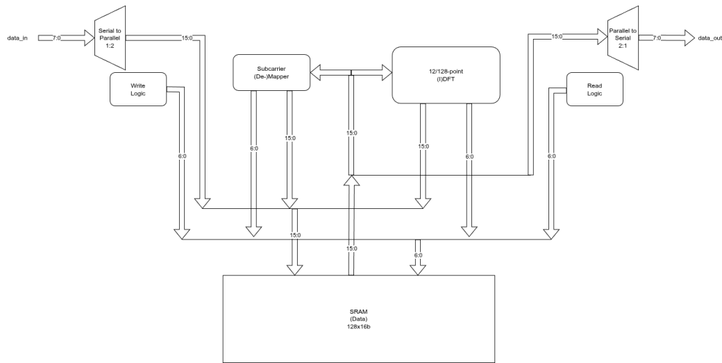
Figure 4: Folded PHY Top Level Architecture
