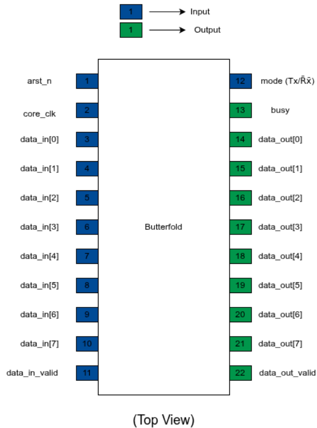
Figure 6: Expected pinout
