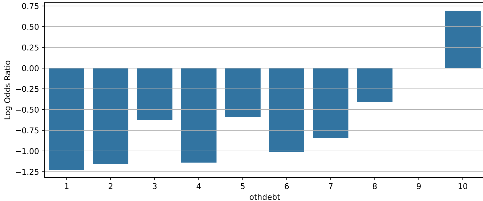
Logit Plot for identifying if the bucketing is required or not for variable othdebt
