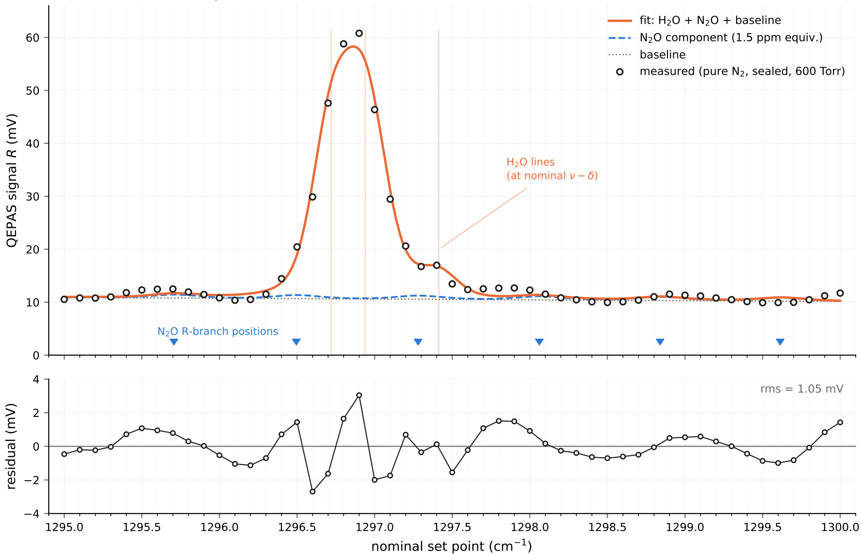
Pure-N 2 scan 28 Jul 2026 vs HITRAN: water fit ( \delta = -0.23 \text{ cm}^{-1} , laser FWHM = 0.26 \text{ cm}^{-1} , R^2 = 0.992 )
