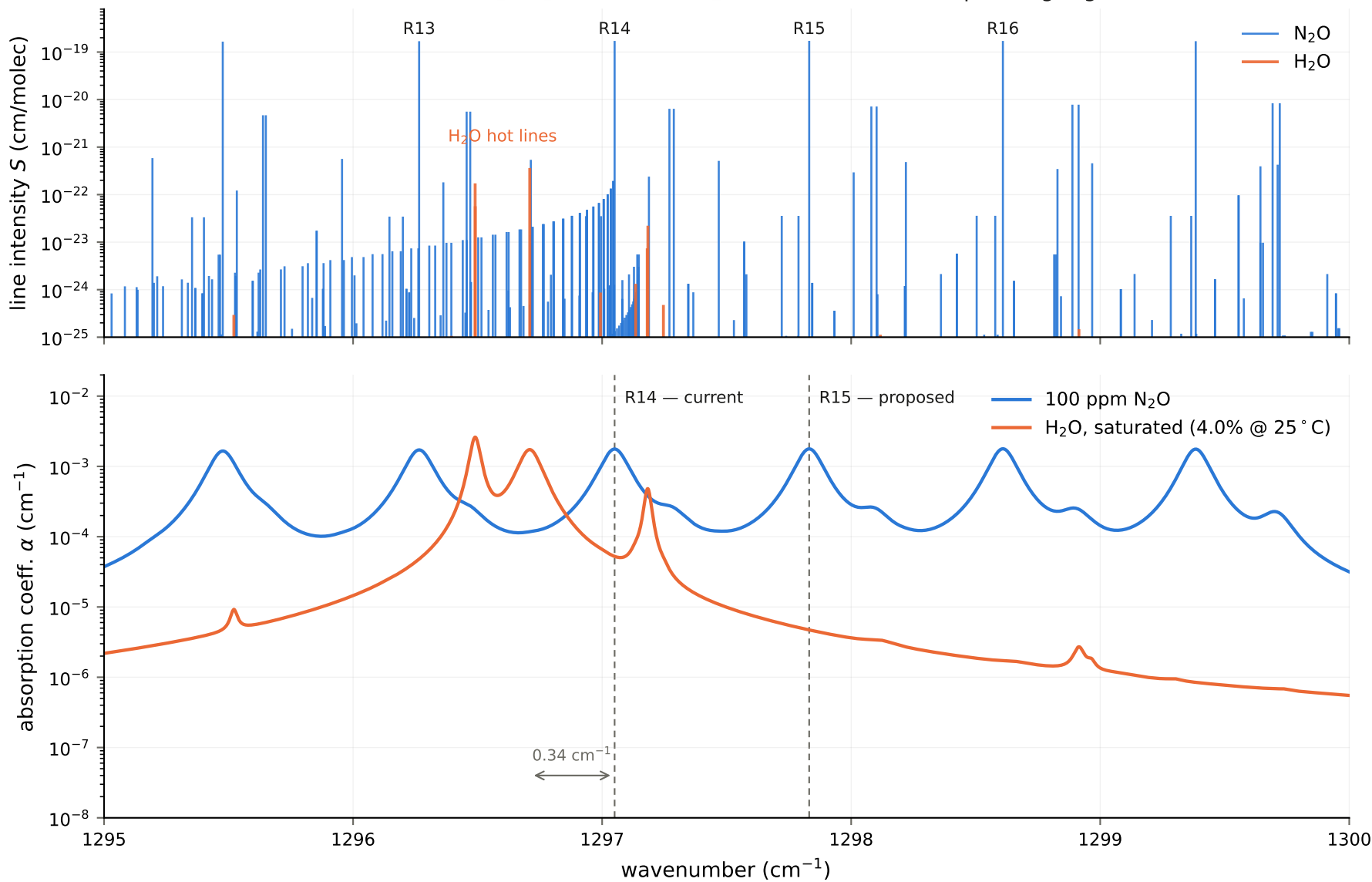
HITRAN 2020: N 2 O \nu_1 R-branch vs H 2 O around the QEPAS operating region
