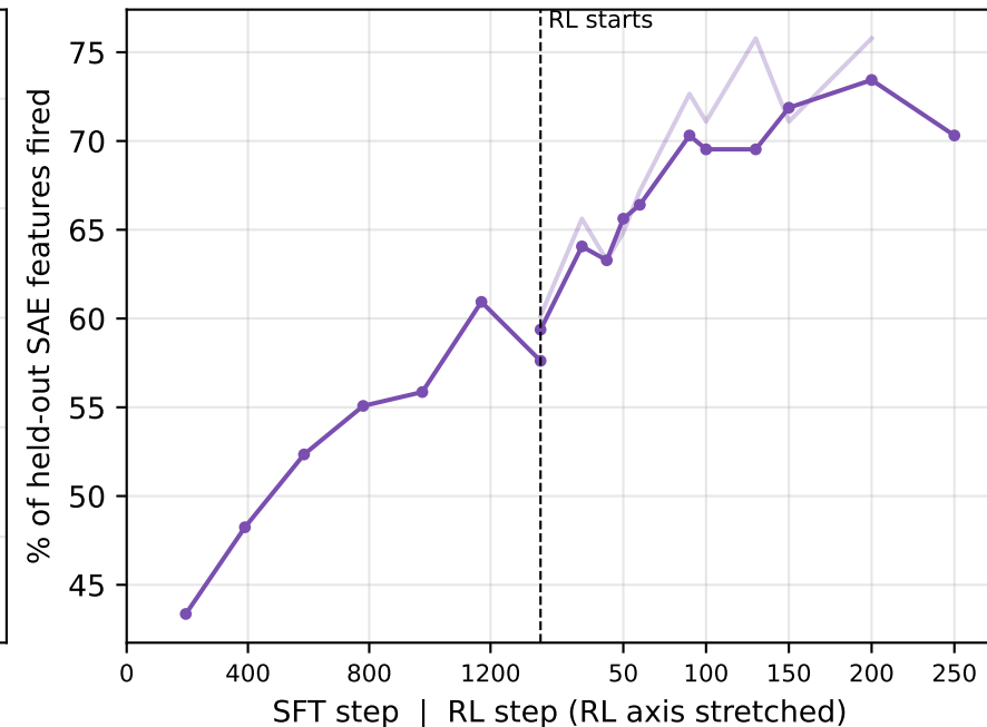
(b) SAE features: target fires
