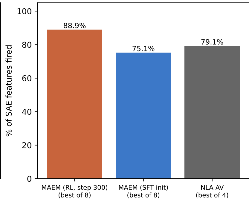
(c) SAE features: target fires
