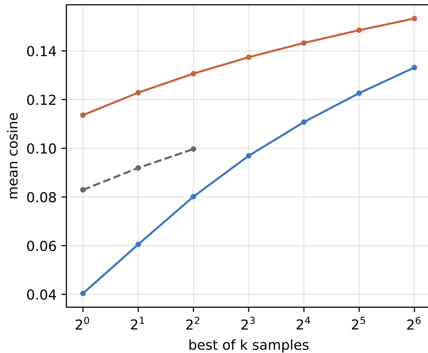
(b) SAE features: cosine
