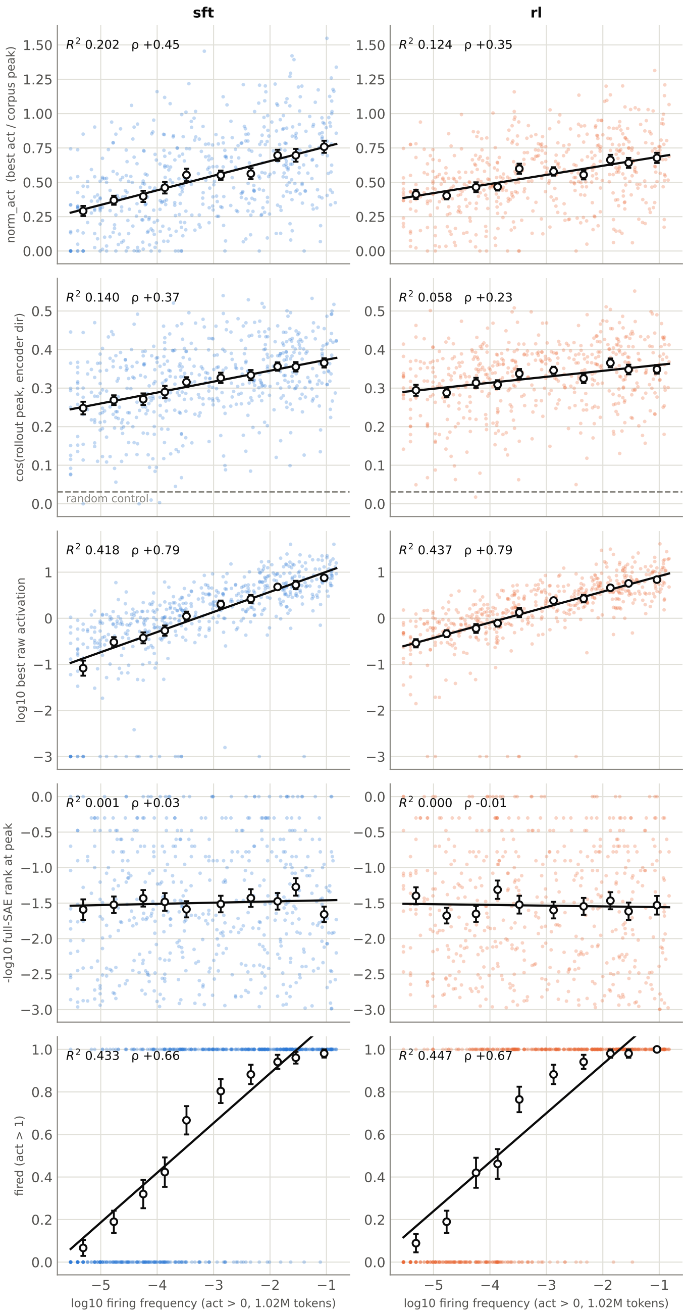
Per-feature recovery vs log10 firing frequency (act > 0, 1.02M tokens)
