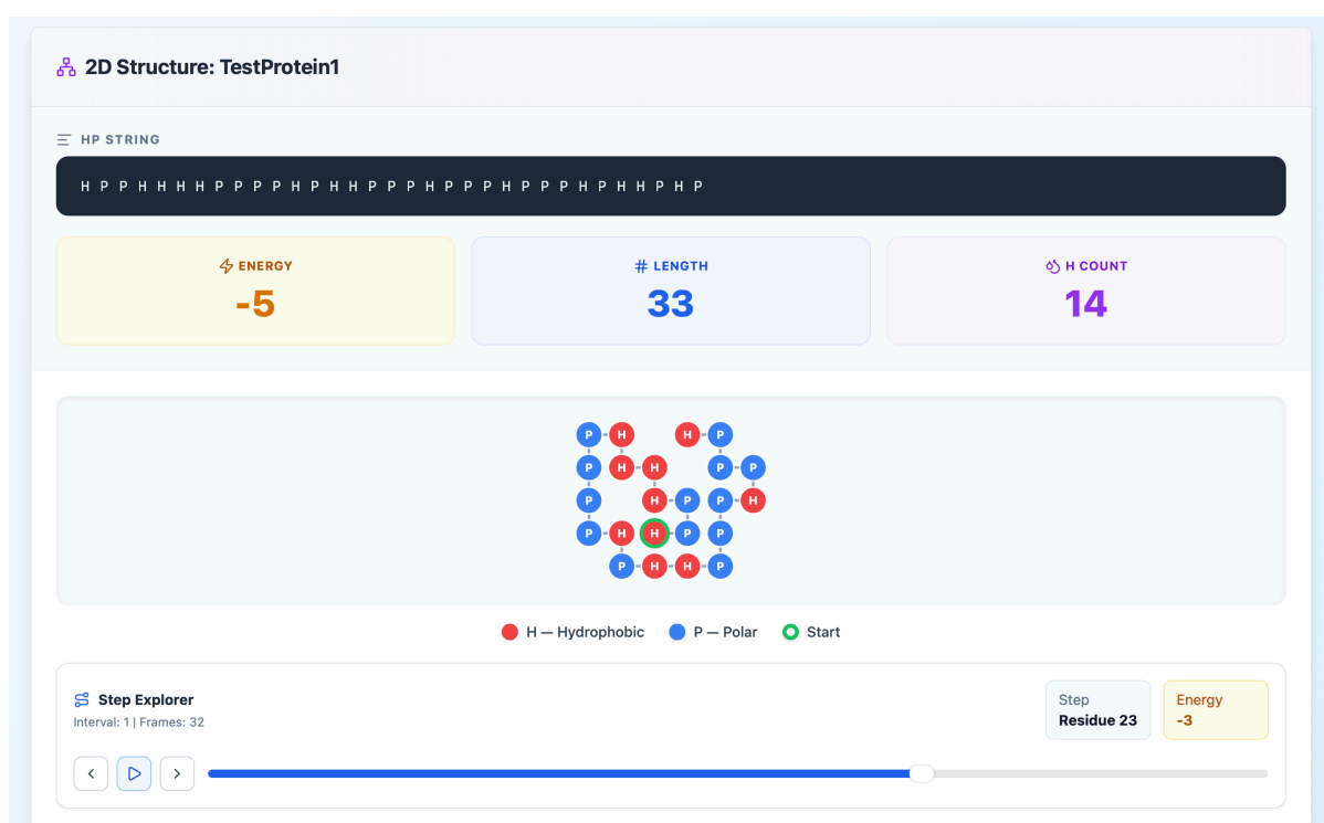
Figure 5.8: Late folding frame in the 2D HP step explorer. The slider position and step counter allow the user to compare this near-final state with earlier conformations.
