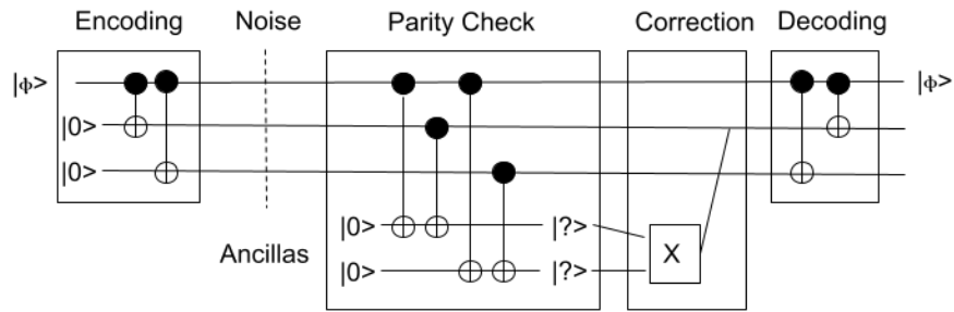
Figure 1: noisy communication via parity measurement, picture from [11]
