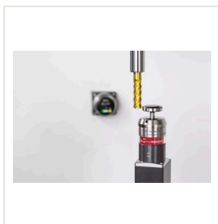
05 Probing & tool breakage
