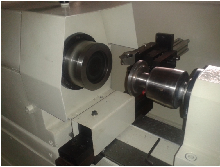
Precision Spindle and Chuck Assembly — Reconditioning Quality Standard
