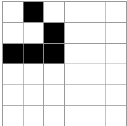
glider, t = 0
