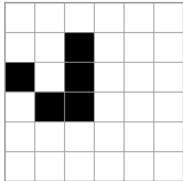
glider, t = 2
