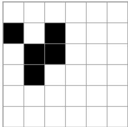
glider, t = 1
