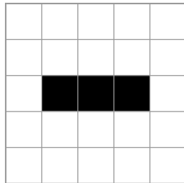
blinker, t = 2
