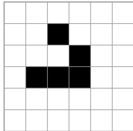
glider, t = 4
