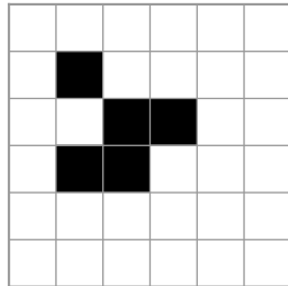
glider, t = 3
