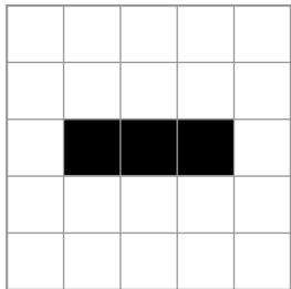
blinker, t = 0
