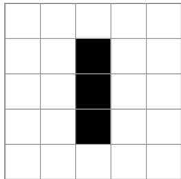
blinker, t = 1
