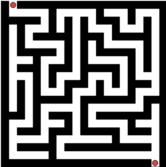
initial maze
