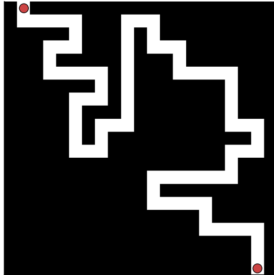
step 50 (solved)
