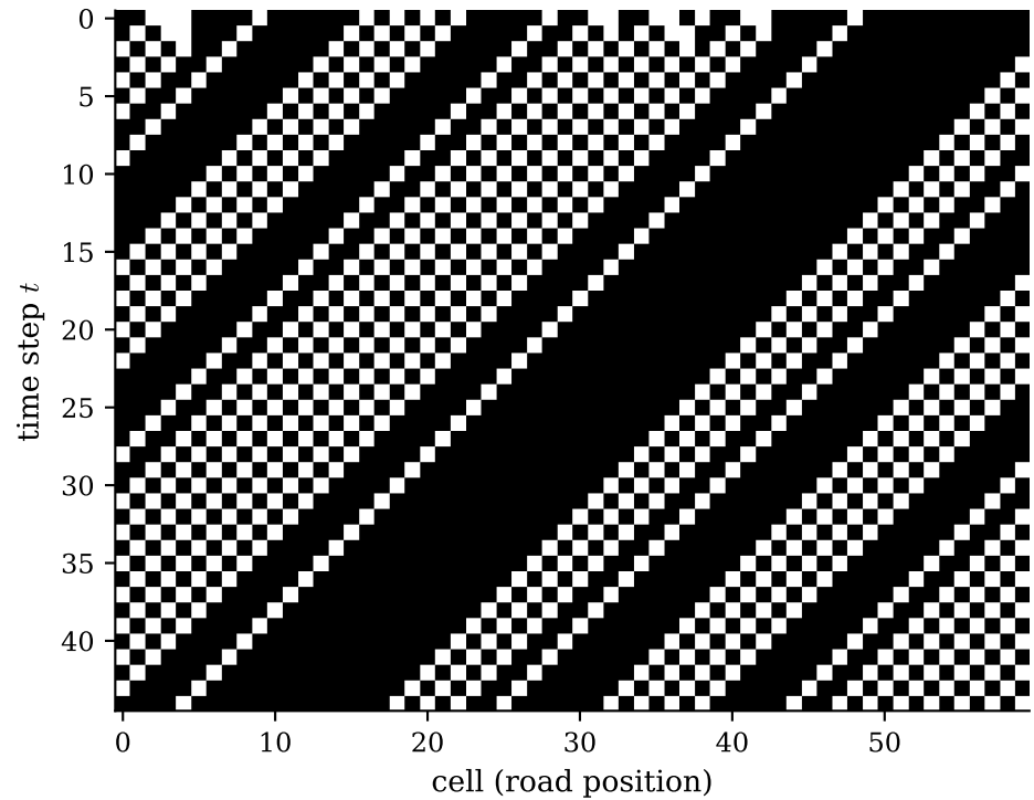
Rule 184, car density \rho = 0.70
