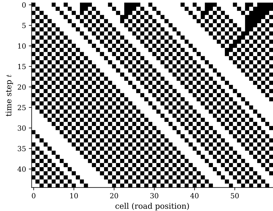
Rule 184, car density \rho = 0.30
