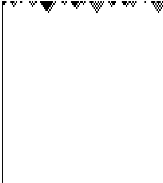
Class 1: rule 160 (homogeneous)
