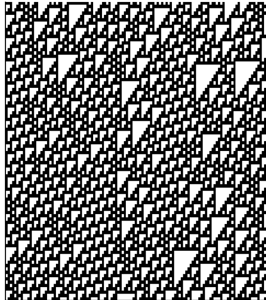
Class 4: rule 110 (localized structures)
