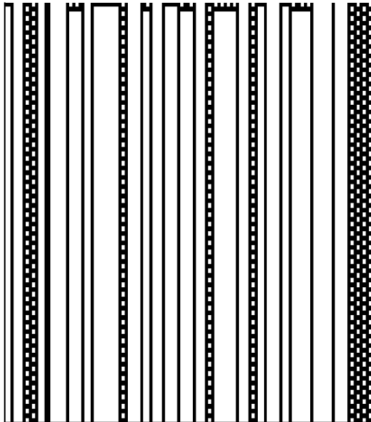
Class 2: rule 108 (periodic)
