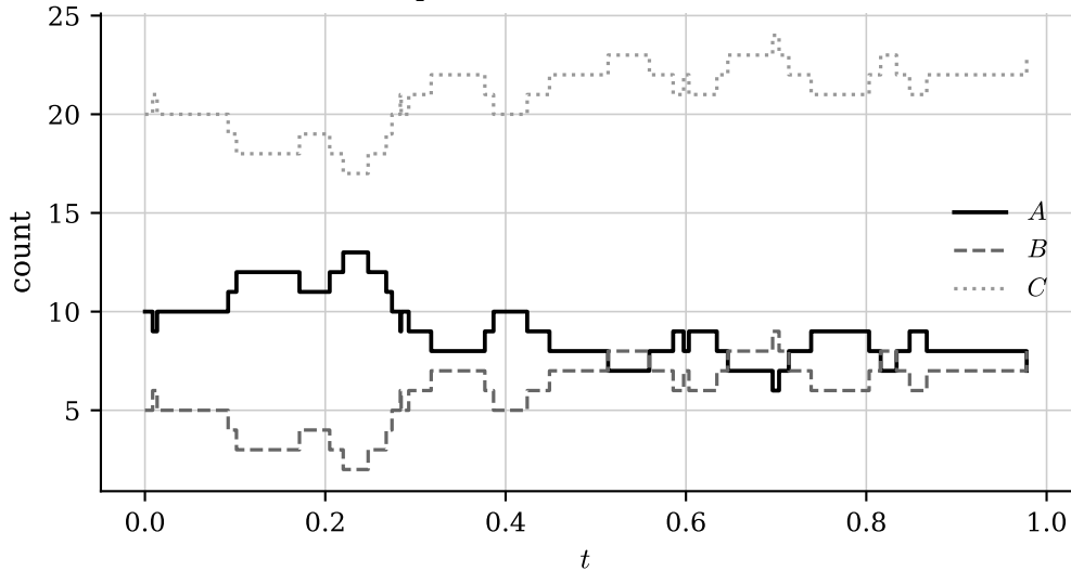
Gillespie SSA staircase ( A \rightleftharpoons B + C )
